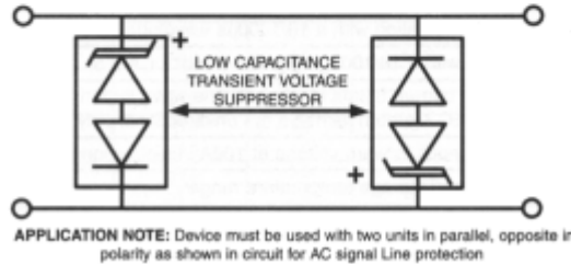
FIG. 4 - AC LINE PROTECTION APPLICATION
